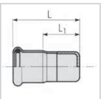
PLUG
