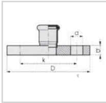
ADAPTER FLANGE
