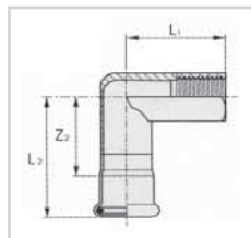
90° FEMALE ANGLE ADAPTER
