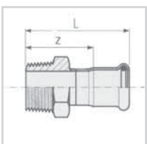
MALE ADAPTER
