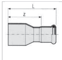
REDUCER
