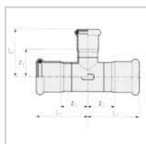
REDUCING-TEE
