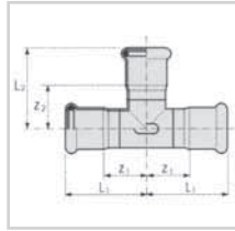
EQUAL-TEE
